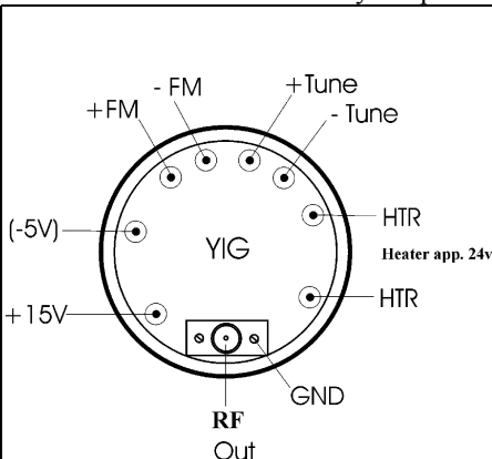
Fig 2: The standard pin connections for a YIG oscillator.
