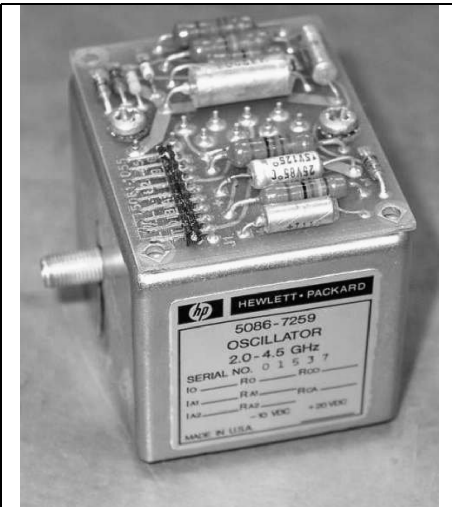
Fig 9: Another example of an HP YIG oscillator.
